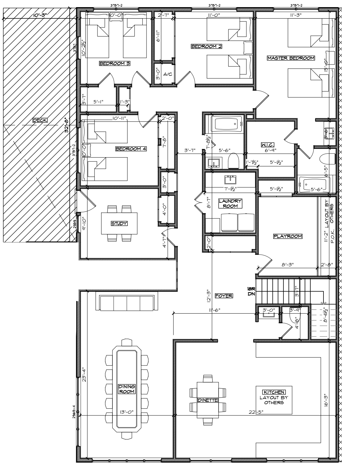
SECOND FLOOR
